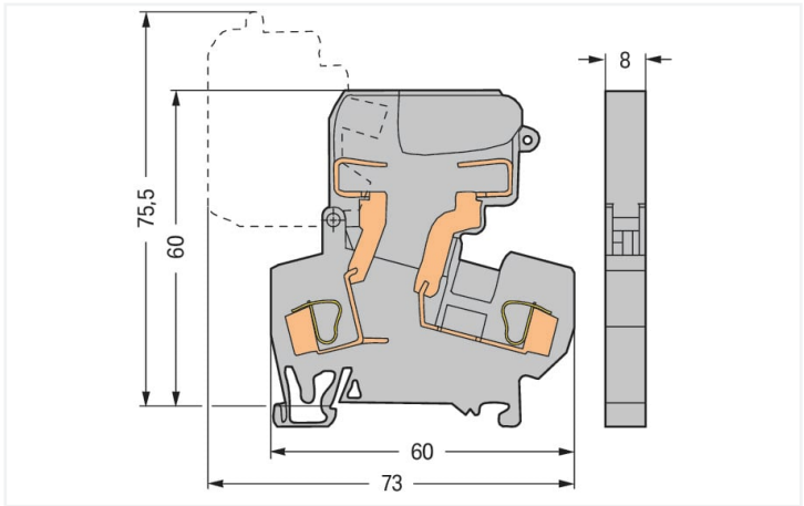
Rozměry v mm Fused disconnect terminal block with a pivoting fuse holder, for (5 x 20) mm glass cart- ridge fuse, without blown fuse indication (281-611)
