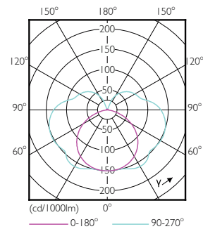
Light Distribution Diagram – CorePro LED linear D 14-120W R7S 118 840
