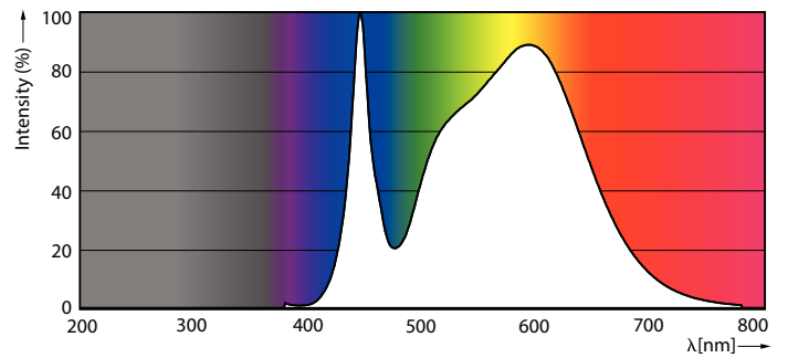
Spectral Power Distribution Colour - CorePro LEDtube 1500mm 20W 840 T8
